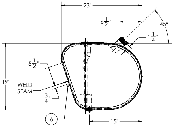
VIEWS FROM LEFT END OF TANK
