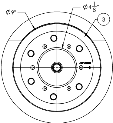
DETAIL A SCALE 1 : 3 GASKET REMOVED FOR CLARITY
