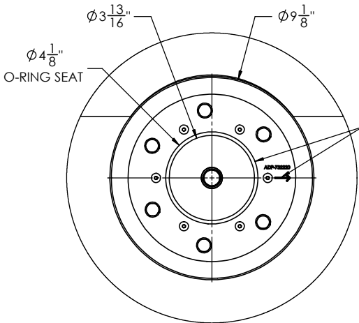
DETAIL A SCALE 1 : 3 GASKET REMOVED FOR CLARITY
