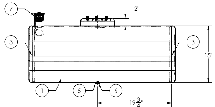
VIEWED FROM LEFT END OF TANK
