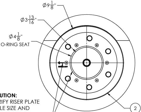
DETAIL A SCALE 1 : 3 GASKET REMOVED FOR CLARITY
