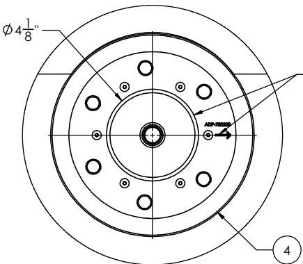
DETAIL A SCALE 1 : 3 GASKET REMOVED FOR CLARITY
