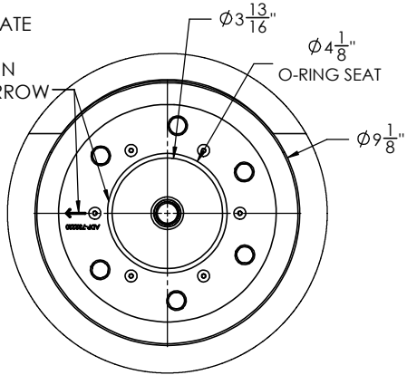
DETAIL A SCALE 1 : 3 GASKET REMOVED FOR CLARITY
