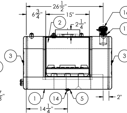
VIEWED FROM RIGHT END OF TANK
