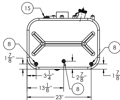
VIEWED FROM LEFT END OF TANK
