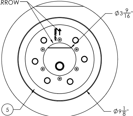
DETAIL A SCALE 1 : 3 GASKET REMOVED FOR CLARITY
